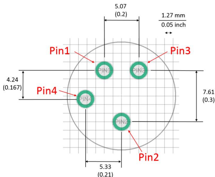
Figure 16: Footprint (dimensions shown in millimeter and inch)
