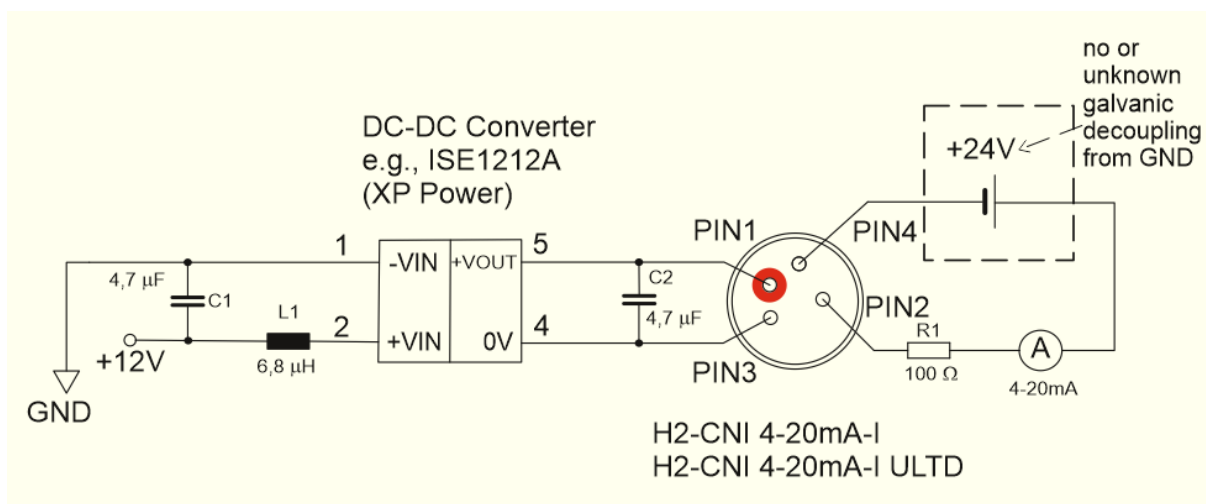
Figure 18: Recommended circuit with DC-DC converter to isolate the supply voltage from ground (GND)
