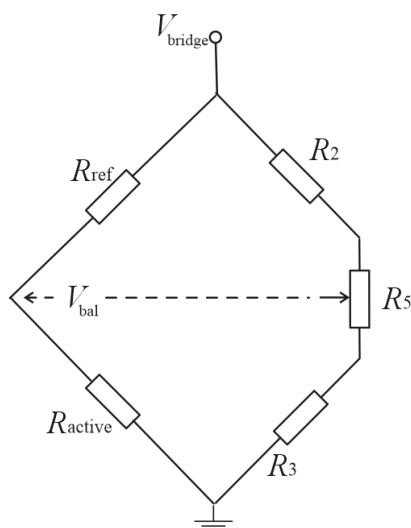
Figure 9. Wheatstone bridge with active and reference sensor element (schematic).
