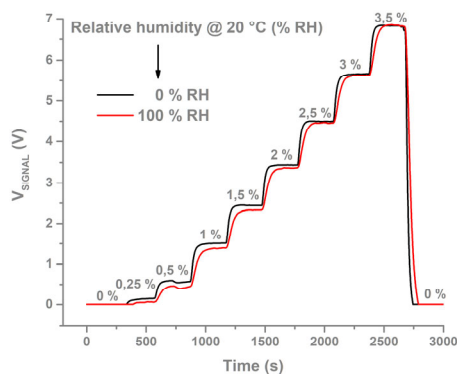
Figure 5. Typical values of the signal transient ( V_{\text{SIGNAL}} ) upon hydrogen exposure at 0 % and 100 % relative humidity (ambient temperature T_a = 20\text{ }^{\circ}\text{C} and a flow of 50 sccm/min).
