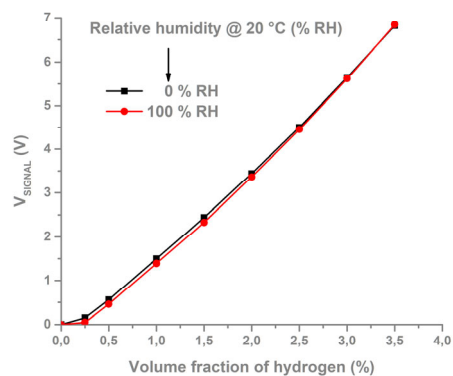
Figure 6. Typical values of the sensor signal ( V_{\text{SIGNAL}} ) as a function of the volume fraction of hydrogen (%) in synthetic air at 0 % and 100 % relative humidity (ambient temperature T_a = 20\text{ }^{\circ}\text{C} , flow of 50 sccm/min).
