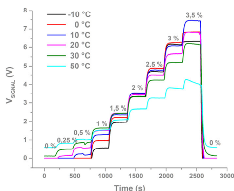
Figure 2. Typical values of the signal transient ( V_{\text{SIGNAL}} ) upon hydrogen exposure in synthetic dry air at different ambient temperatures between -10\text{ °C} and 50\text{ °C} and a total flow of 50 sccm/min.
