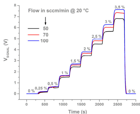
Figure 8. Typical values of the signal transient ( V_{\text{SIGNAL}} ) upon hydrogen exposure in synthetic dry air at different flows of 50, 70 and 100 sccm/min (ambient temperature T_a = 20^\circ\text{C} ).
