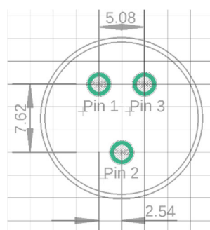
Figure 10: Footprint (dimensions shown in millimeter)
